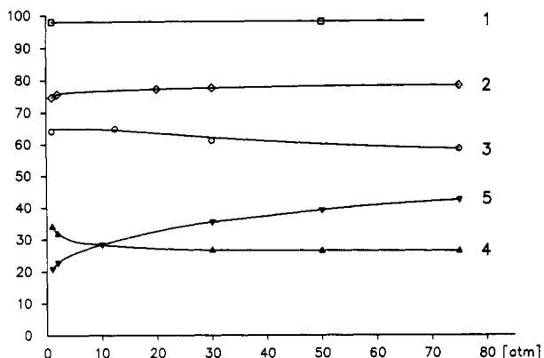
Figure 5. Dependence of the optical yield (percent) on the H_2 pressure (atm) for the 1–5 catalyzed hydrogenation of \alpha -(acetylaminocinnamic acid at room temperature (22 °C).
